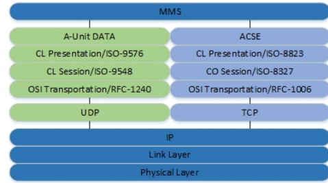
Fig. 4: The protocol layers of MMS over TCP and UDP [12]
