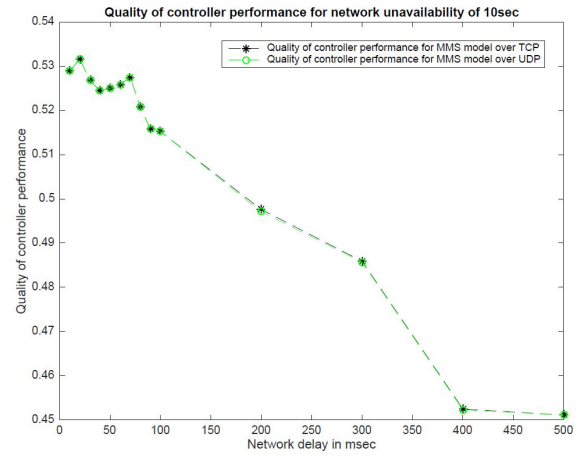
Fig. 8: Quality of controller performance with 5 TCP connection losses for 10 Sec.
