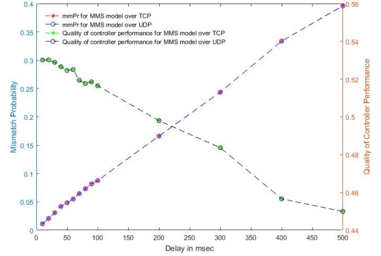
Fig. 6: Assessment of mmPr for different network delays
