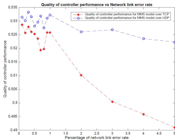
Fig. 10: Quality of controller performance for different link errors
