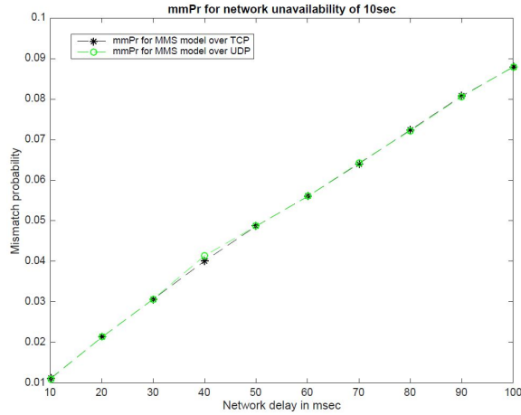
Fig. 7: mmPr with network unavailability of 10 Sec. for 5 times
