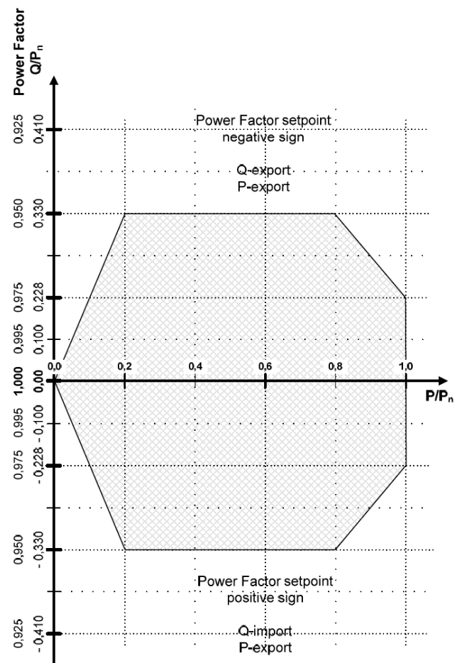
Figure 10. P-Q/Pmax-profile for WPPs [6]
