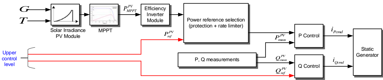
Figure 48. Overview of the PVP Model
