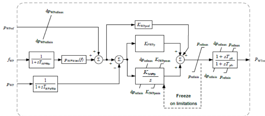
Figure 47: WPP active power controller [20]
