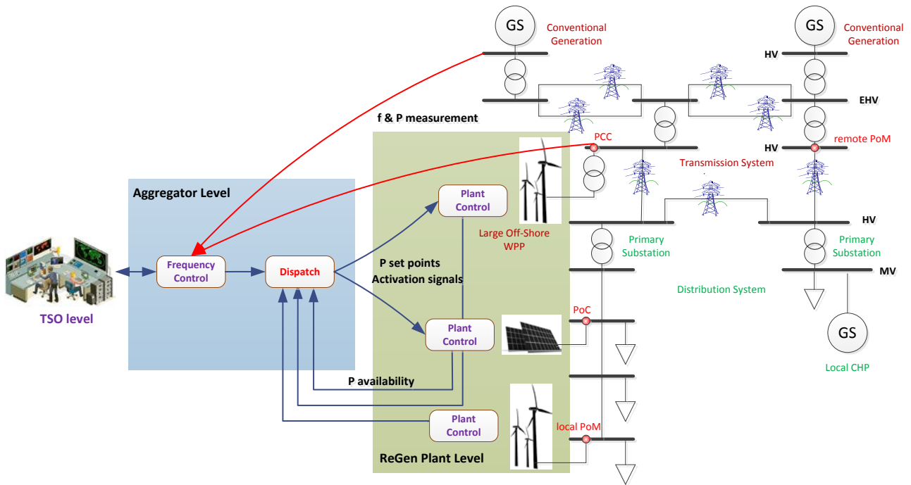
Figure 30. Control coordination by means of frequency control
