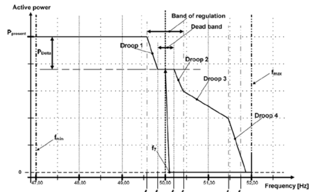
Figure 18. Frequency control for WPPs and PVPs with small downward regulation [6] [7]
