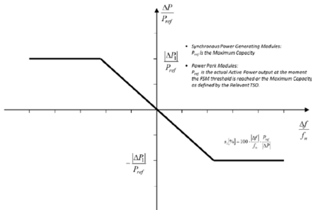
Figure 16. Active power response capability with zero deadband [4]
