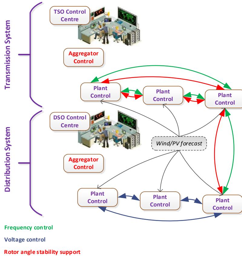
Figure 27. Decentralized Control Architecture
