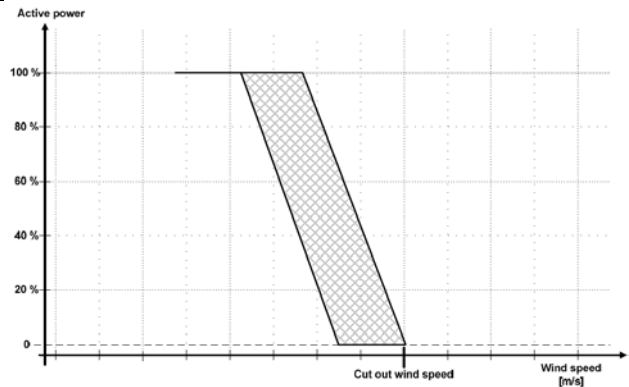
Figure 22. Downward regulation of active power at high wind speeds [6]
