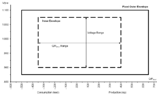
Figure 6. U-Q/Pmax-profile [4]
