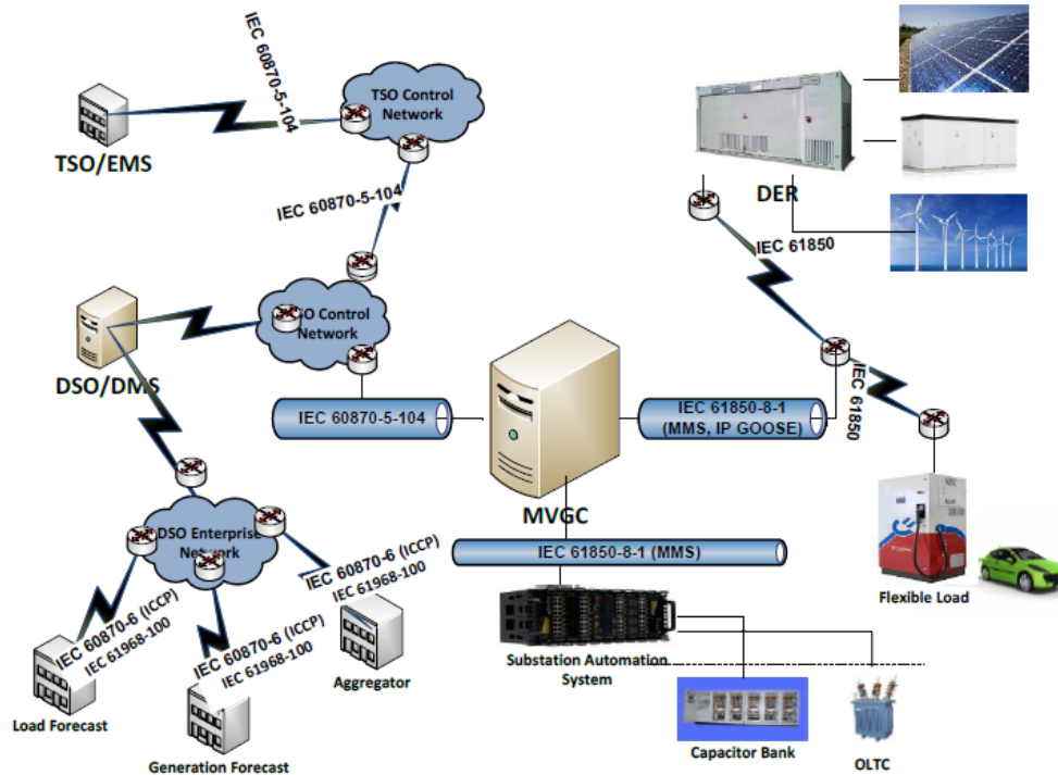
Figure 51 Overview of Standard Protocols [2]
