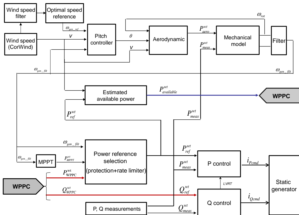
Figure 43: Overview of the WTG model.
