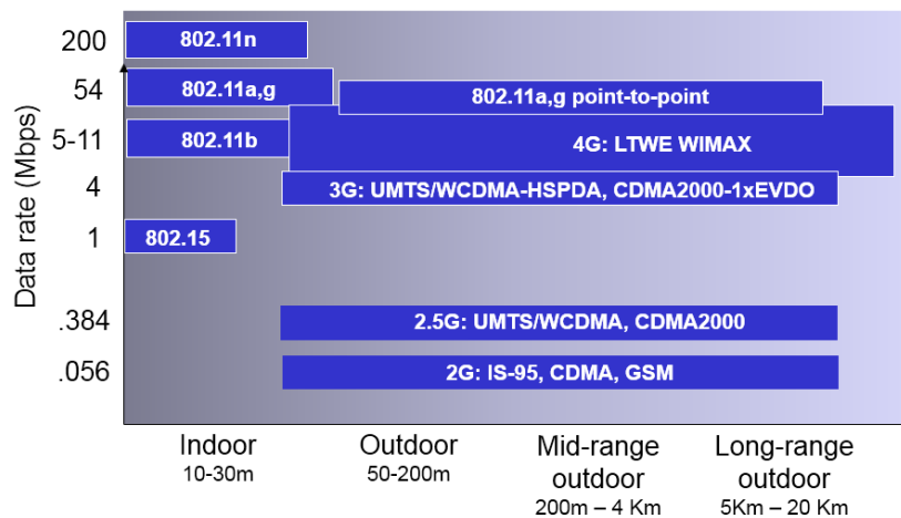
Figure 43 Characteristics of Selected Wireless Link [22]
