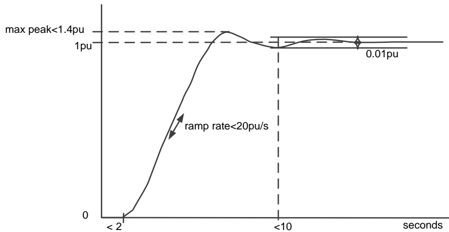
Figure 33. Requirement for reactive power performance
