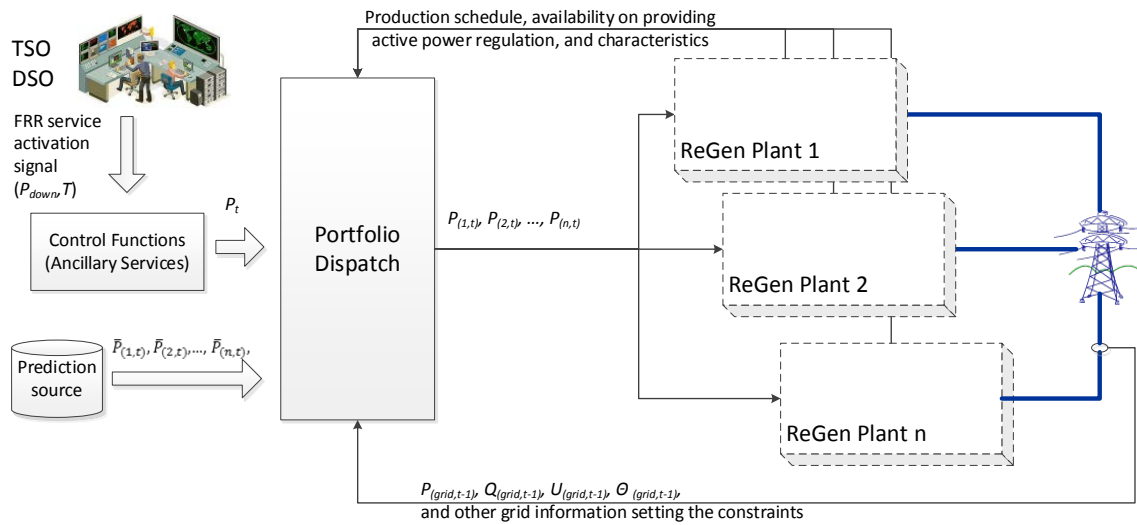
Figure 32. Flow chart of secondary frequency control
