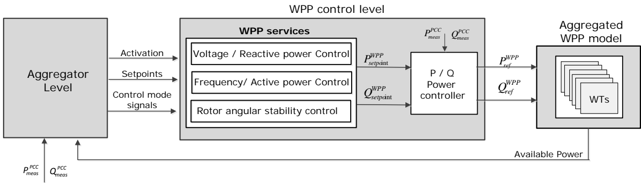
Figure 45: WPP control level.
