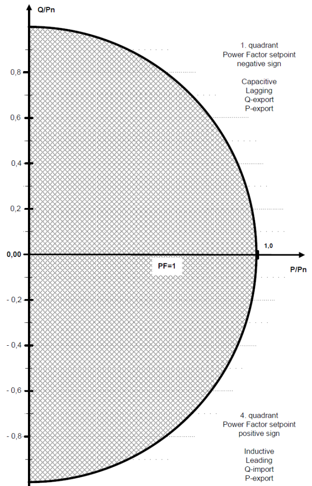
Figure 12. P-Q/Pmax-profile for PVPs [7]
