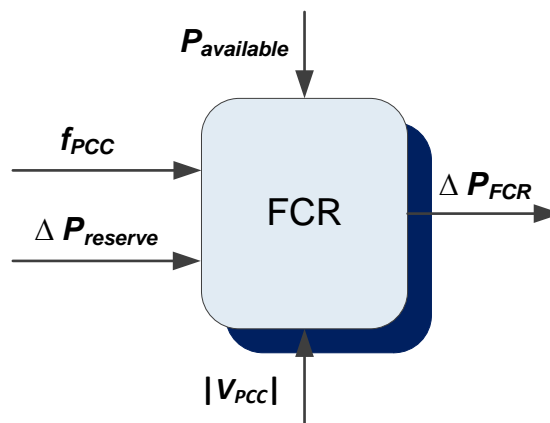
Figure 39: Frequency Control Functional Specification
