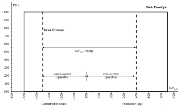
Figure 7. P-Q/Pmax-profile [4]
