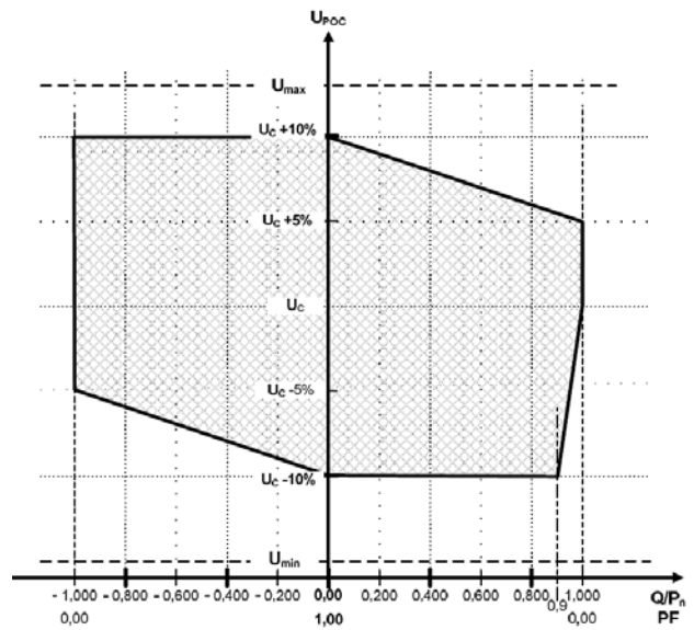
Figure 11. U-Q/Pmax-profile for PVPs [7]
