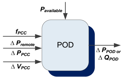
Figure 42: Frequency Restoration Reserve Functional Specification.
