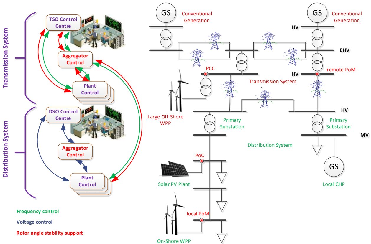
Figure 25. General control architecture including power system & assets and control levels
