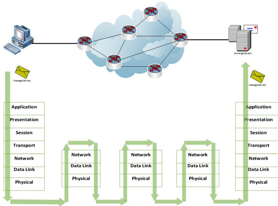
Figure 50 Signal Flow through Layered Architecture
