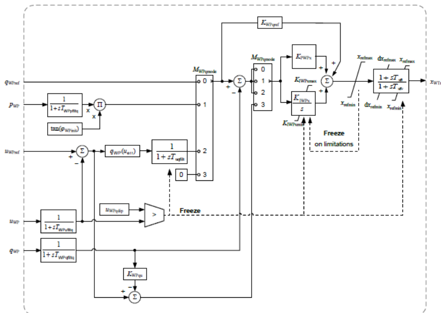
Figure 46: WPP reactive power controller [20]
