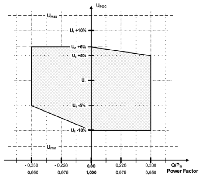
Figure 9. U-Q/Pmax-profile for WPPs [7]
