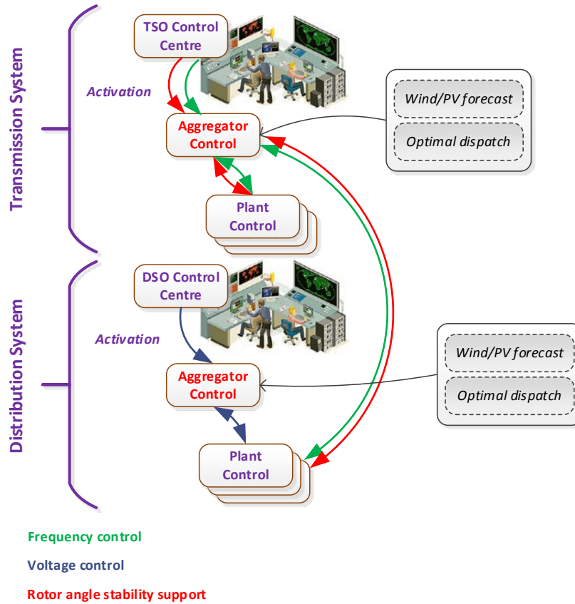
Figure 26. Centralized Control Architecture
