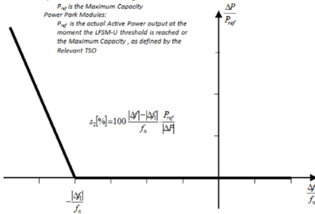
Figure 15. LFSM-U [4]
