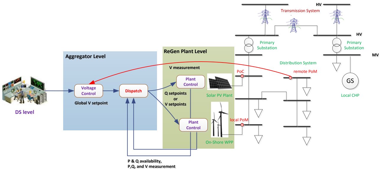
Figure 29. Control coordination by means of voltage control
