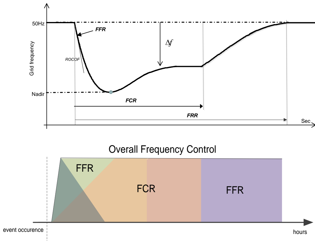
Figure 35: Frequency response contribution stages from ReGen
