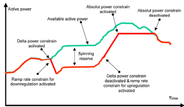
Figure 23. Constraint functions for active power [6] [7]
