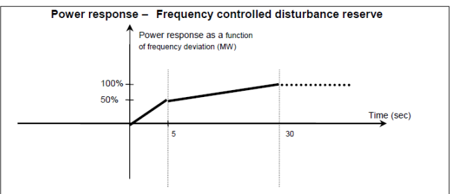
Figure 21. Frequency-controlled normal operation and disturbance reserve applicable for Eastern Danish power system [9]
