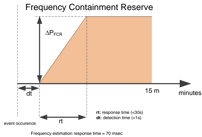
Figure 38: Frequency Containment Reserve Specifications
