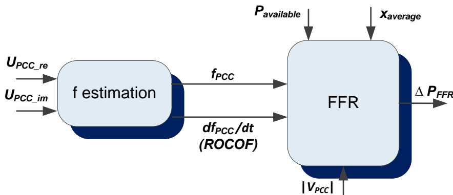
Figure 37: Frequency response Functional Specification
