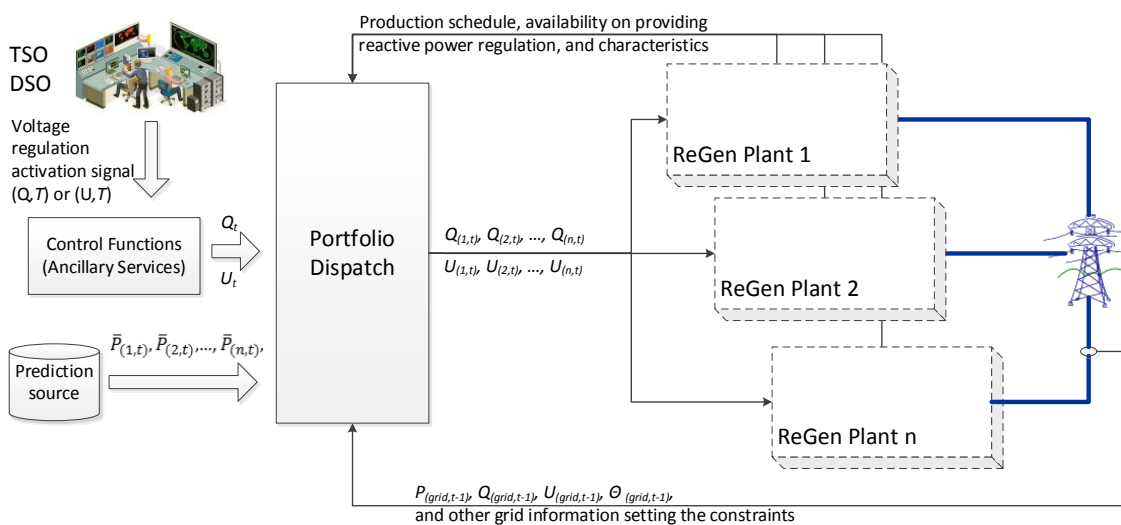
Figure 31. Flow chart of reactive power control.
