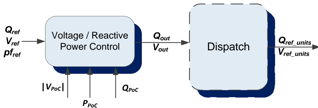
Figure 34. Voltage / Reactive Power Control: Functional description
