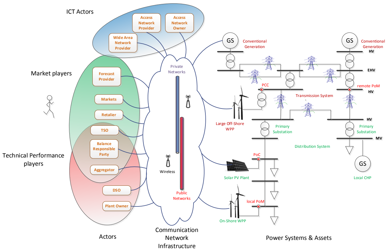
Figure 1. General system architecture including power system & assets, control levels, ICT layer and actors
