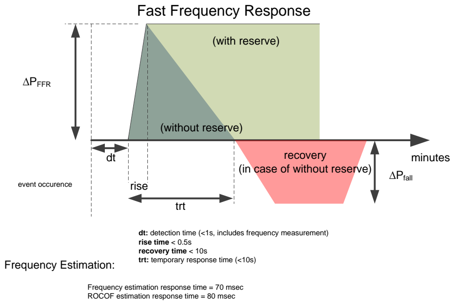
Figure 36: Fast frequency response Design Specification
