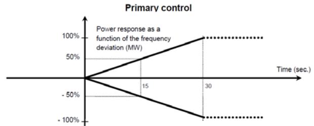
Figure 20. Primary frequency control applicable for Western Danish power system [9]
