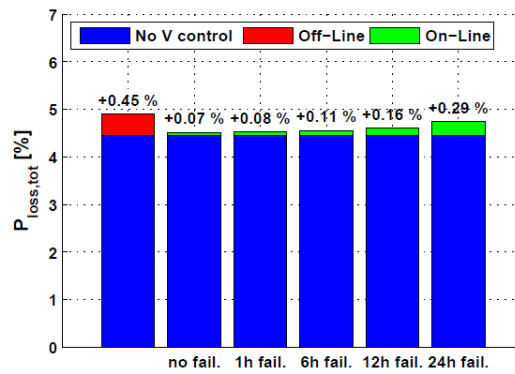
Fig. 4. Average power losses over the simulation period for various durations of communication failure for updating the voltage set-points
